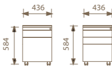
Pedestals / Caissons Prof. / Depth : 590 or 790 mm.
